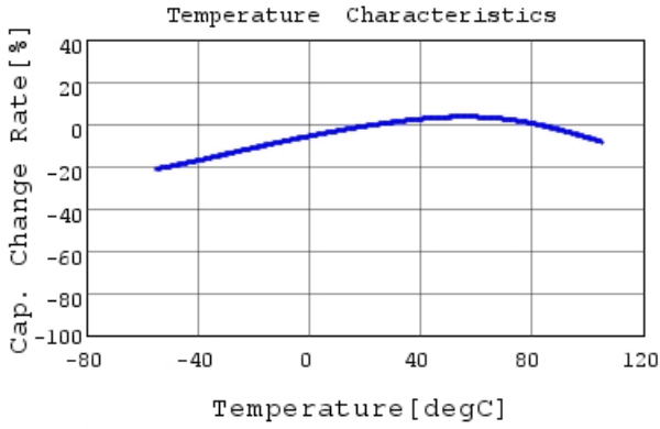
GRM21BC8YA106KE11 C-Temp. capchange, DC0.0V,
