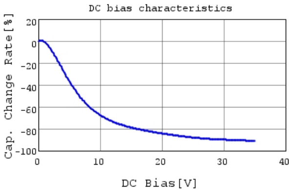
GRM21BC8YA106KE11 C-DC bias capchange, 25.0c
