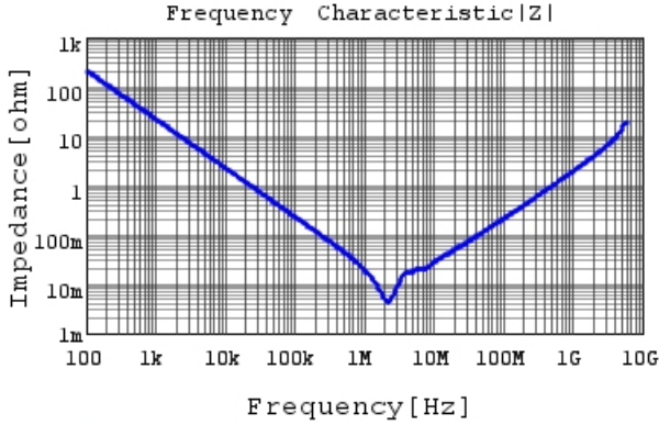
GRM21BC8YA106KE11 |Z| DCOV,25degC
