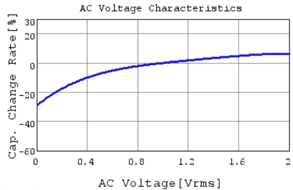
GRM21BC8YA106KE11 C-AC Voltage capchange, Dc
