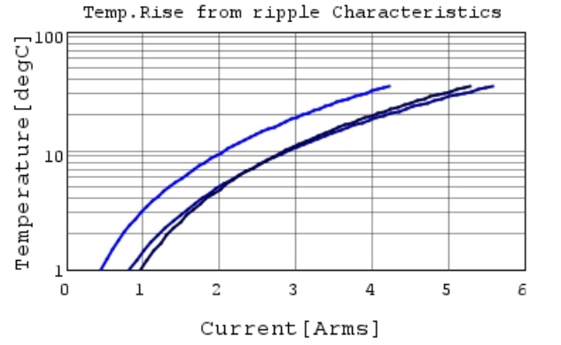
GRM21BC8YA106KE11 Temp.rise — 80kHz —
