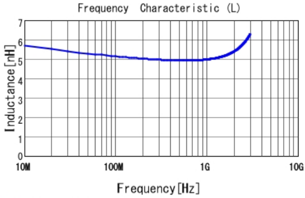
■ LQG15HN5N1S02 L
