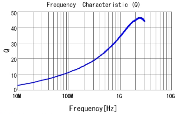
■ LQG15HN5N1S02 Q
