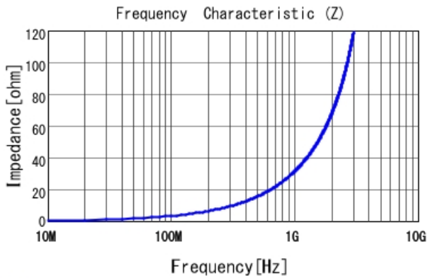
■ LQG15HN5N1S02 |Z|
