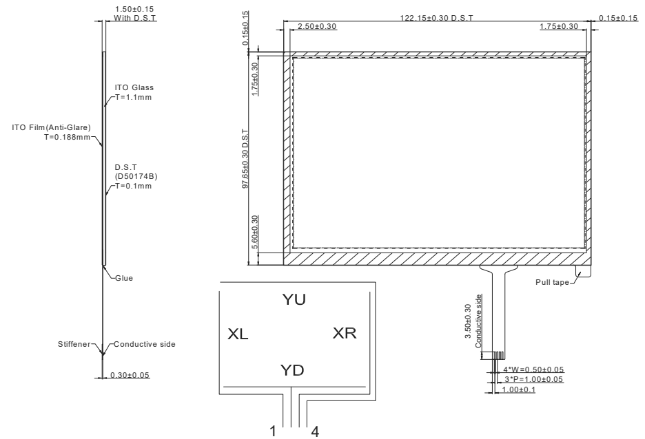
TOUCH PANEL PIN ASSIGNMENT
