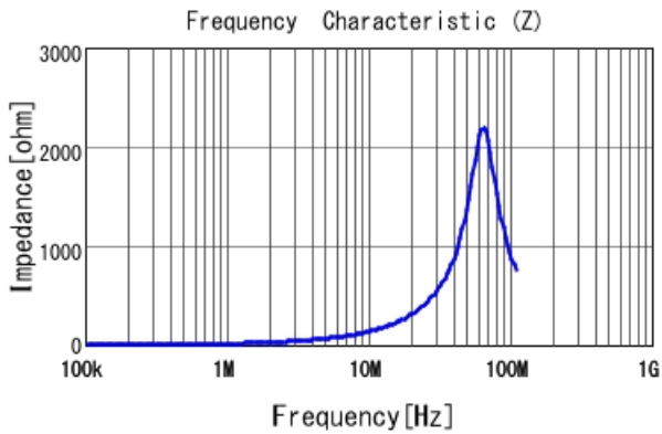
LQM31PN2R2M00 |Z|
