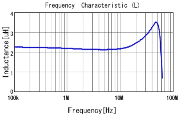
LQM31PN2R2M00 L
