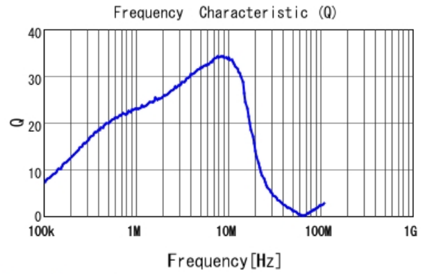
LQM31PN2R2M00 Q
