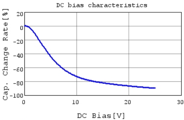
GRM188C81E475KE11 C-DC bias capchange, 25.0c
