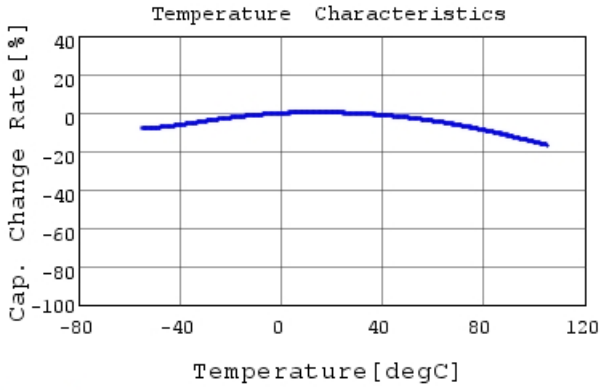
GRM188C81E475KE11 C-Temp. capchange, DC0.0V,
