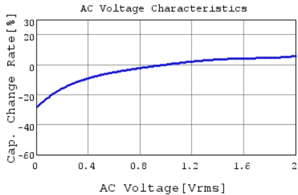
GRM188C81E475KE11 C-AC Voltage capchange, Dc
