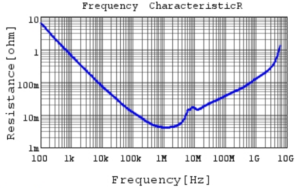
GRM188C81E475KE11 R DCOV, 25degC
