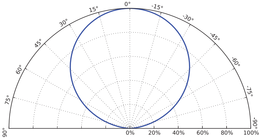
Figure 6. Typical polar radiation pattern for LUXEON 2835 with FreshFocus Technology at 120mA, T J =25°C.
