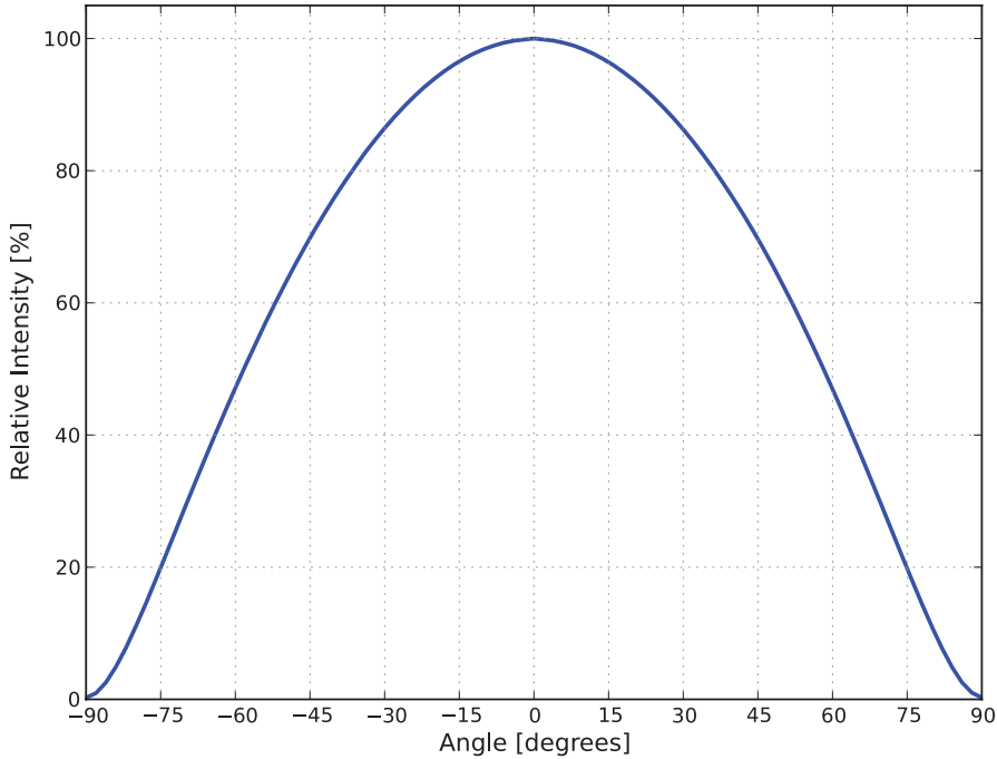
Figure 5. Typical radiation pattern for LUXEON 2835 with FreshFocus Technology at 120mA, T J =25°C.
