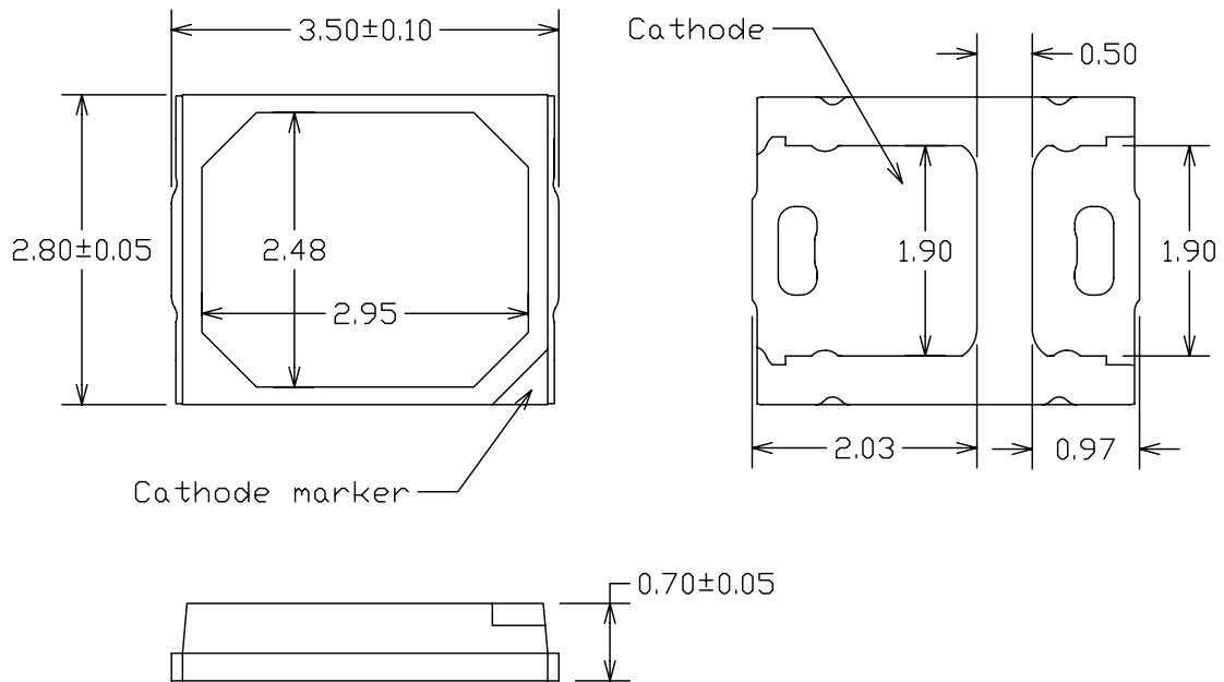
Figure 9. Mechanical dimensions for LUXEON 2835 with FreshFocus Technology.
