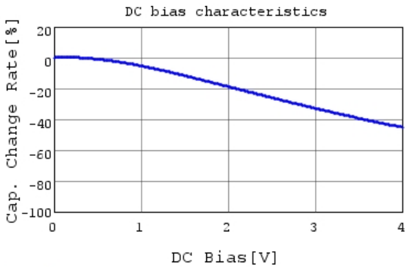
GRM32EE70G107ME19 C-DC bias capchange, 25.0c
