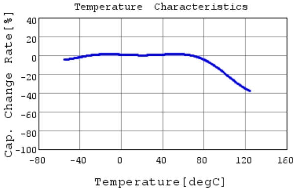
GRM32EE70G107ME19 C-Temp. capchange, DC0.0V,
