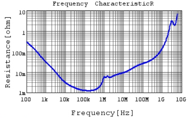
GRM32EE70G107ME19 R DCOV, 25degC
